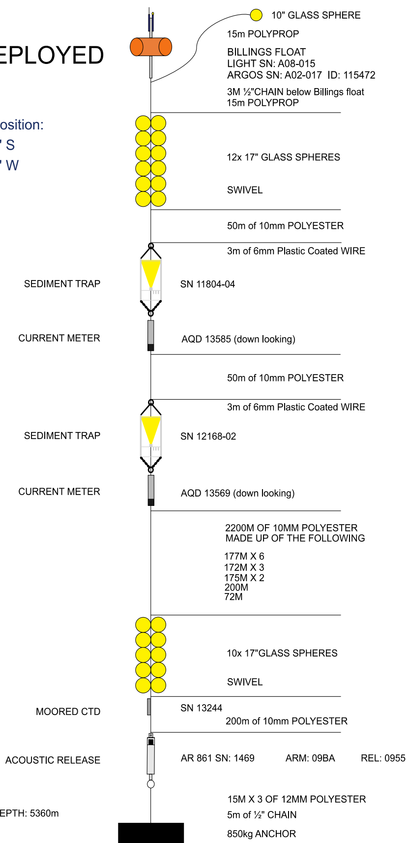
Figure 1: SOG mooring as deployed in 2017
