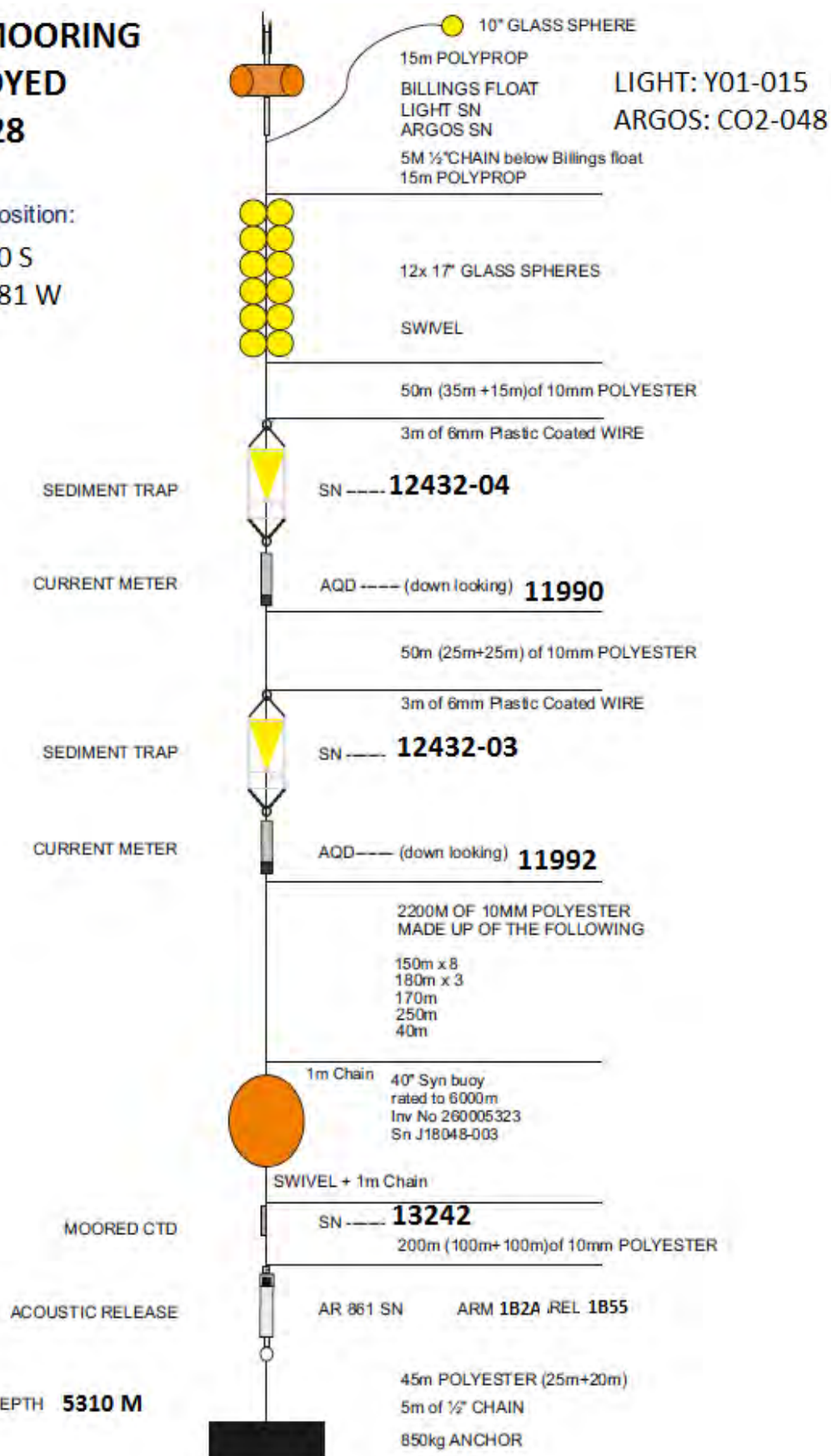
Figure 5: SOG mooring as deployed on AMT28 in 2018
