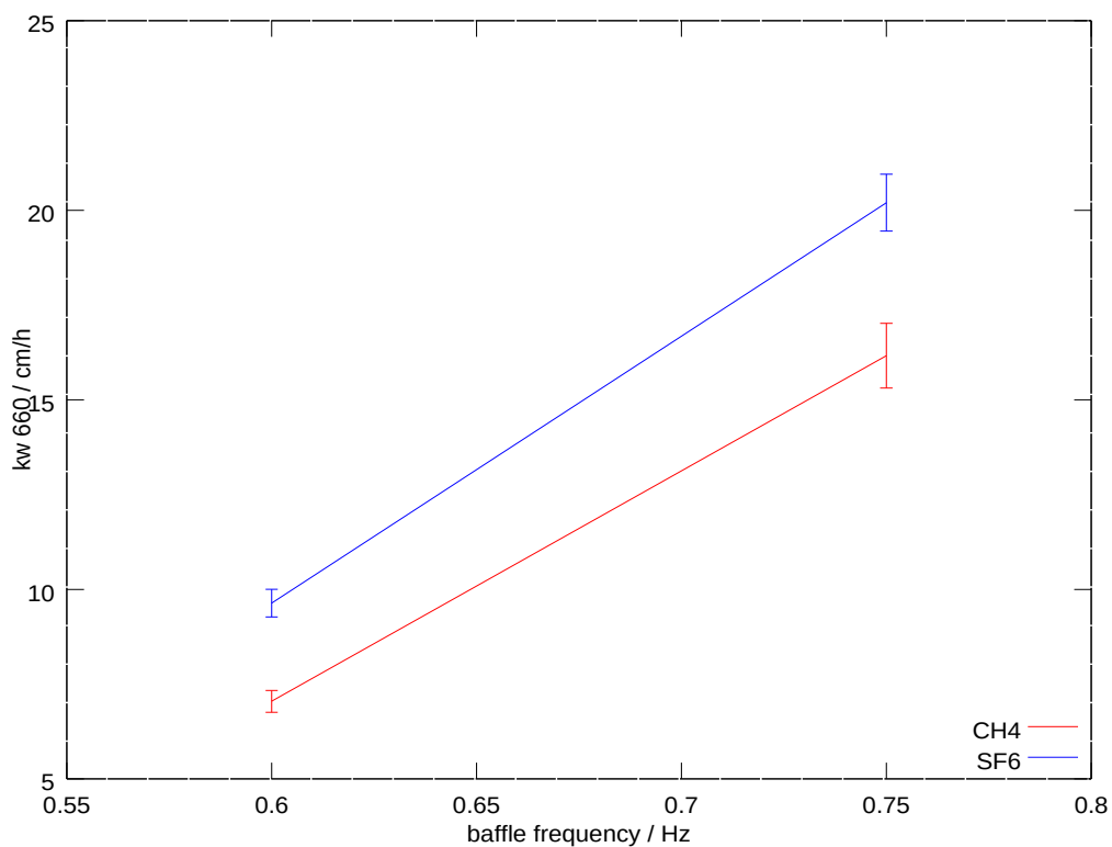
Figure 1: Gas transfer velocities ( k_w ) of CH 4 and SF 6 normalised to 660 Schmidt number for two baffle speeds (0.6 and 0.75 Hz) derived from water samples collected from the underway system at CTD_S024. Error bars (better than 5%) are calculated from GC standards run before and after a sample run.
