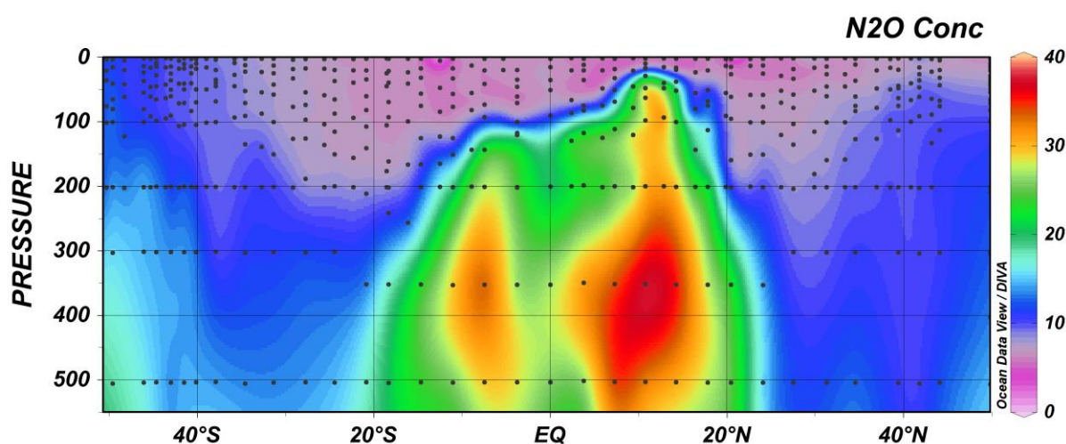
N 2 O concentration (nmol L -1 ) during AMT24, September-November 2013
