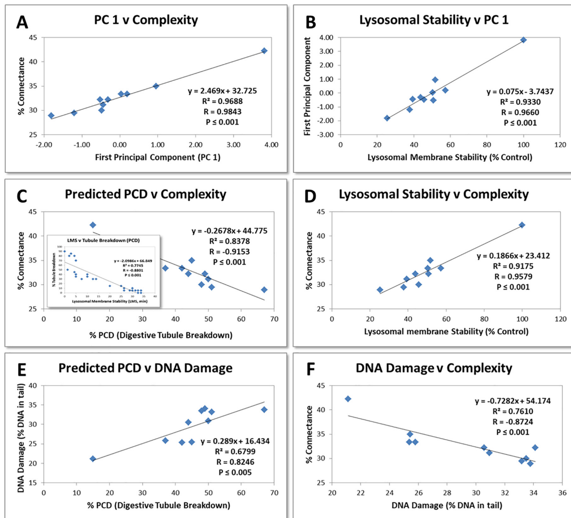
Fig. 8. Statistical modelling of system complexity ( C_0 ), lysosomal stability, predicted programmed cell death and DNA damage based on C_{60} and BaP biomarker data (including data for 0.01 and 0.1 mg/L C_{60} ) versus: A. first principal component (PC 1) v complexity; B. Lysosomal membrane stability (LMS) versus PC 1; DNA damage (Comet); C. Predicted programmed cell death (PCD) v complexity (Inset: – LMS v digestive tubule breakdown as indicator of PCD); D. lysosomal stability versus complexity; and E. Predicted programmed cell death (PCD) versus DNA damage; and F. DNA damage versus complexity. Coefficient of determination ( R^2 ), Pearson's correlation coefficient ( R ), and probability values (one-tailed test).
