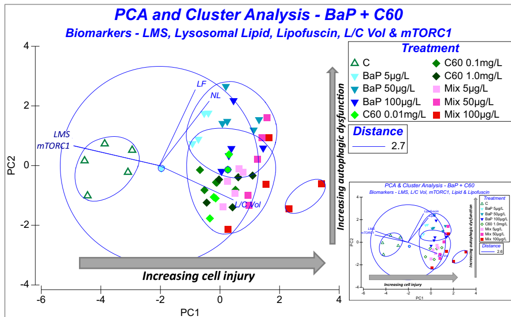
Fig. 6. Principal component (PCA) and cluster analysis of the C 60 and BaP biomarker data not including DNA damage, but including data for 0.01 and 0.1 mg/L C 60 . Vectors indicate the directionality of specific biomarkers. Arrows indicate: a. Increasing Cell Injury corresponding to the first principal component (PC1); and b. Increasing trend for Autophagic Dysfunction based on elevated intralysosomal lipofuscin and lipid, and corresponding to the second principal component (PC2). Inset: PCA excluding data for 0.01 and 0.1 mg/L C 60 . Vectors: LMS – lysosomal membrane stability; L/C Vol – lysosome/cell volume ratio (autophagy biomarker); LF – lysosomal lipofuscin (lipofuscinosis); NL – lysosomal lipid (lipidosis); and mTORC1 – phosphorylated mTORC1.
