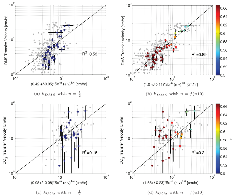
Figure 2. Ninety-minute averaged k and the prediction of the small-eddy model based on measured \epsilon taken within the uppermost 0.5 m ( \epsilon_{0.5} ) of the ocean in log–log space. The color code represents n , the errors bars show the standard error of k ( \text{std}/\text{sample size}^{1/2} ), the grey data in the background are the non-averaged data, and the dashed line represents the 1:1 relation.
