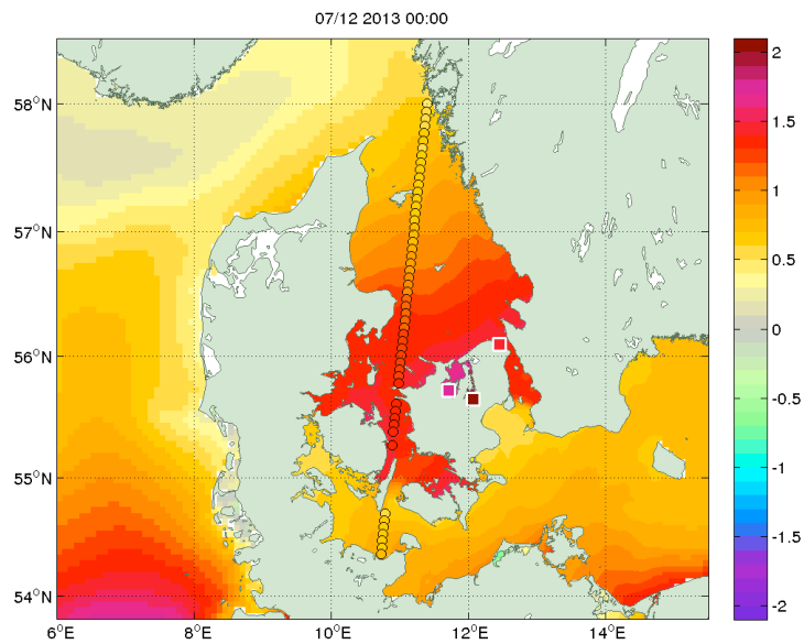
Figure 4 Example of satellite altimetry verification of model performance. Cryosat-2 observations (filled circles) and tide gauge observations (filled squares) are overlaid the Danish Meteorological Institute (DMI) storm surge model field. The surge occurred during the Bodil storm 6-7 December 2013 and resulted in a 1000 years event in Roskilde, Denmark. Source: Generated by co-author J. Høyer.
