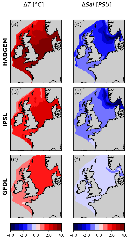
Figure 2. Surface temperature and salinity; difference between future (2070–2099) and present (1990–2019) periods.
