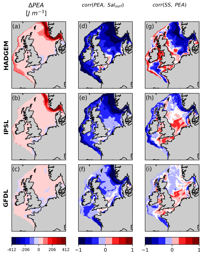
Figure 6. Change in potential energy anomaly (PEA) and correlation between PEA and surface salinity and PEA and SS. White areas on the shelf indicate non-significant correlation.
