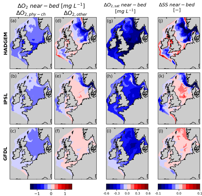
Figure 4. Contributions of near-bed oxygen change, \Delta O_{2,phy-ch} and \Delta O_{2,other} , and changes in SS and O_{2,sat} . Note that the spatial distribution of \Delta O_{2,sat} and \Delta SS closely follows that of \Delta O_{2,phy-ch} and \Delta O_{2,other} respectively.
