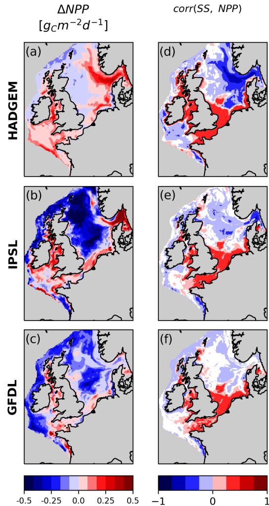
Figure 7. Change in depth-integrated net primary production (NPP) and correlation between NPP and SS. White areas on the shelf indicate non-significant correlation.
