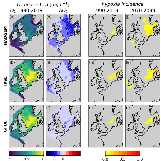
Figure 3. Near-bed O_2 concentration, present state (average of 1990–2019), and change (difference of the 2070–2099 and 1990–2019 averages) and fraction of year with average near-bed oxygen < 6 \text{ mg L}^{-1} under present-day and future conditions, calculated on bias-corrected data. Hatched regions in panels (d), (e) and (f) are deoxygenation hotspots.
