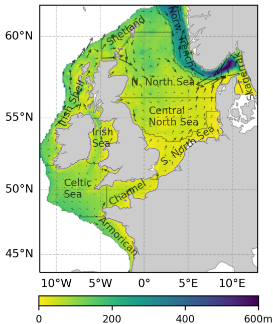
Figure 1. The northwest European continental shelf and its sub-basins considered in this study. Colour scale represents bathymetry. Arrows indicate the mean annual circulation for the sample year 2000.
