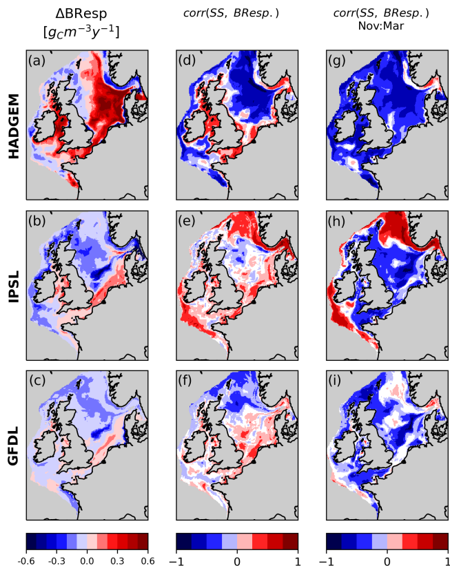
Figure 8. Change in near-bed BResp and correlation between BResp and SS for all months and for months from November to March alone. White areas on the shelf indicate non-significant correlation.
