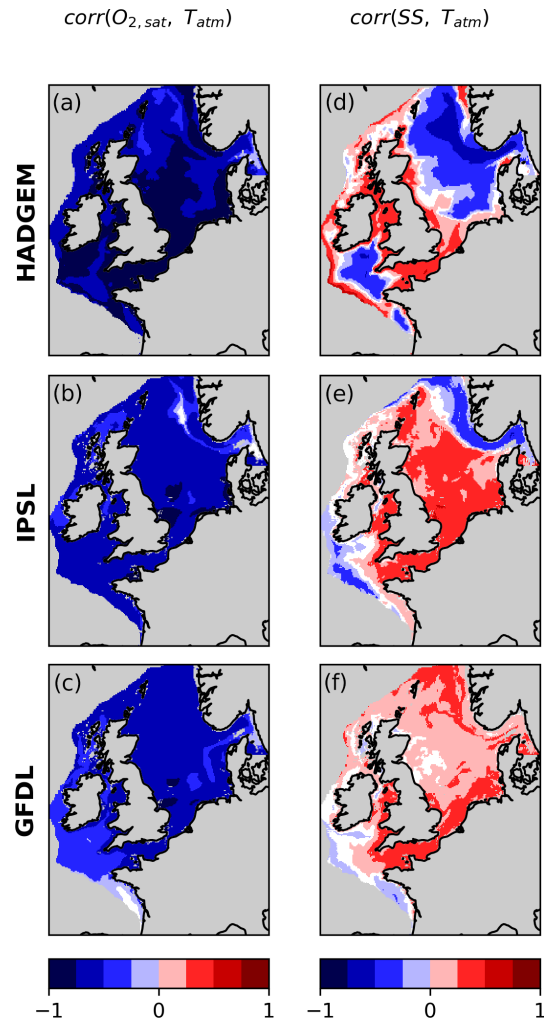
Figure 5. Correlation between temperature atmospheric forcing and near-bed O_{2,sat} and SS. White areas on the shelf indicate non-significant correlation.
