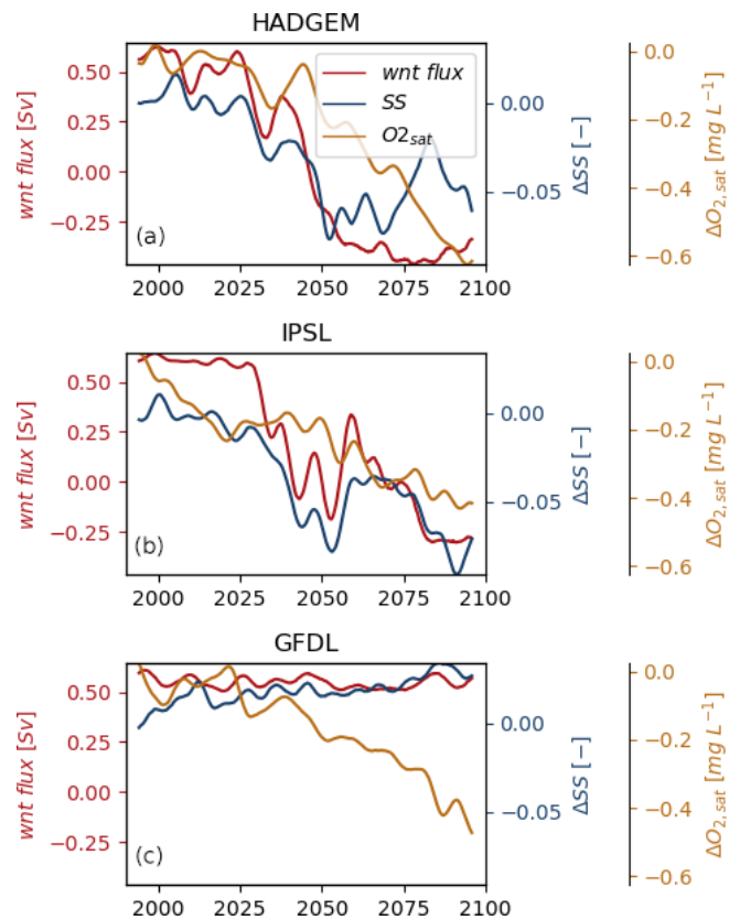
Figure 9. Temporal evolution of \Delta SS and \Delta O_{2,sat} in the Norwegian trench and western Norwegian trench current flux; monthly average data are smoothed with a Gaussian filter. Positive values of the current are entering the North Sea.
