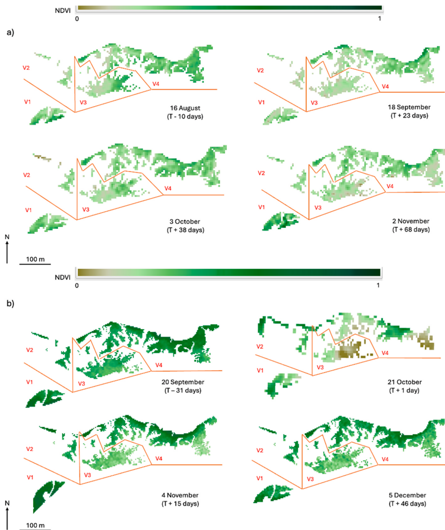
Fig. 4. NDVI for St John's Lake saltmarsh (S1) in a) 2016 (Rapid Eye data) and b) 2021 (Planet Scope data except for 21 October which was Rapid Eye data hence the lower resolution). Images show subsites V1 to V4 with boundaries in red correlating to Fig. 1c and d. (For interpretation of the references to colour in this figure legend, the reader is referred to the Web version of this article.)
