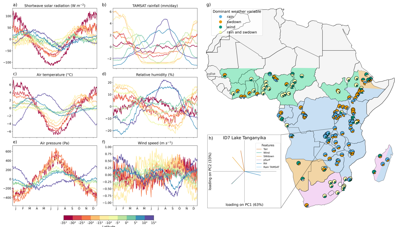
Fig. 3 | Seasonality and Principal Components of atmospheric variables. a–f Climatological year showing the average seasonal evolution of atmospheric variables in lakes across latitudes (colorbar). Each line represents the climatological data, with the annual mean removed, and averaged across lakes within the same latitude range. Climatologies for all variables considered in this study for each lake are available in Table S.2 in the Supplementary Materials. g Lake clusters based on climate variables predominantly explained by the first two principal components
