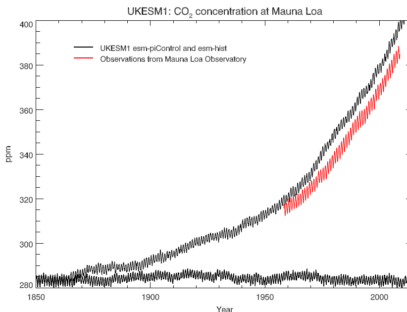
Figure C2. Monthly time series of near-surface CO 2 at Mauna Loa, Hawaii, from UKESM1 emission-driven piControl and historical experiments, and CDIAC observations.
