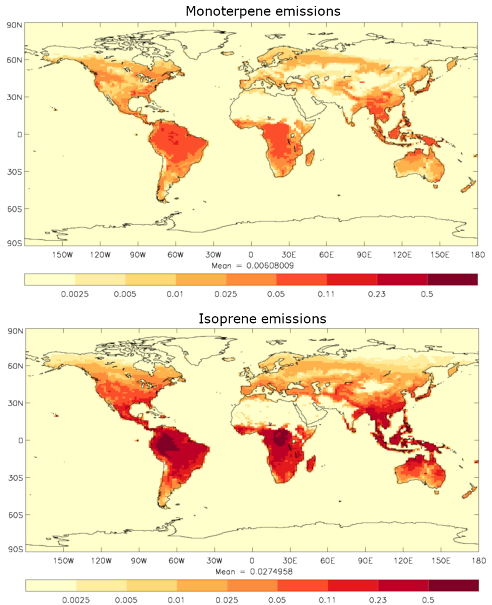
Figure 25. Annual mean emissions ( \text{TgC year}^{-1} ) of monoterpenes (top) and isoprene (bottom) from the UKESM1 historical simulations (2005–2014).
