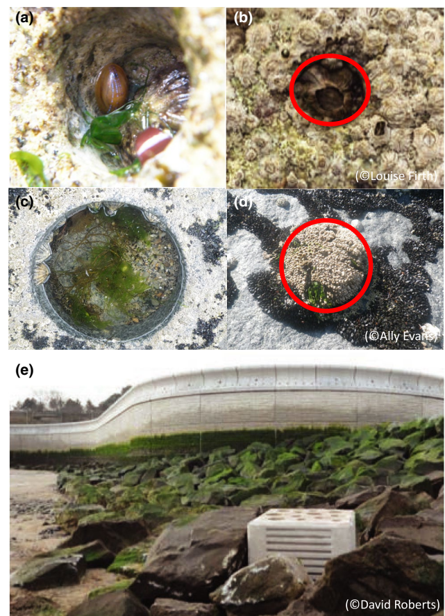
FIGURE 2 Unintended outcomes from integrated greening of grey infrastructure experiments. Drilled pits after 5 (a) and 9 years (b); longer term observations revealed that many (red circle indicates outline) had become dominated by individual barnacles. (c) Drilled rockpools after 1.5 (c) and 5 years (d); longer term observations revealed that some rockpools (red circle indicates outline) filled up with the worm Sabellaria alveolata . (e) The BIOBLOCK is a habitat-enhancement unit. Following 2013/14 storms, the BIOBLOCK became covered by sand and it was still buried in 2019. All examples from Firth et al. (2014)
