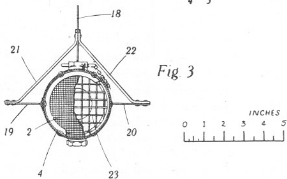
FIGS. 1, 2 and 3.—Showing respectively a plan, a longitudinal and a transverse optical section of the Plankton Indicator. For detailed description and references to letters and numbers see text.
