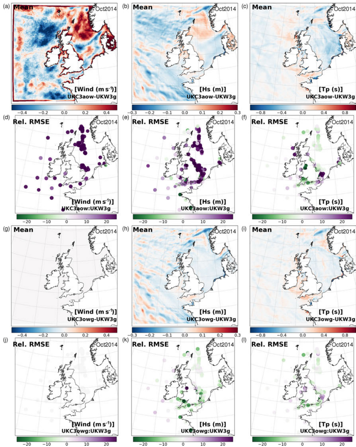
Figure 5. Sensitivity of wave model wind forcing, significant wave height ( H_s ) and peak wave period ( T_p ) to coupling during October 2014 experiment. Monthly mean differences between UKC3aow and UKW3g for (a) coupled/forced atmosphere winds, (b) significant wave height H_s and (c) peak wave period T_p . (d–f) Percentage difference in RMSE statistic for UKC3aow results relative to UKW3g for (d) wind forcing, (e) H_s , (f) T_p . (g–i) Monthly mean differences between partially coupled UKC3owg and UKW3g (i.e. with same global-scale wind forcing) for (g) wind forcing, (h) H_s , (i) T_p , and (j–l) percentage difference in RMSE statistics for each variable for UKC3owg relative to UKW3g.
