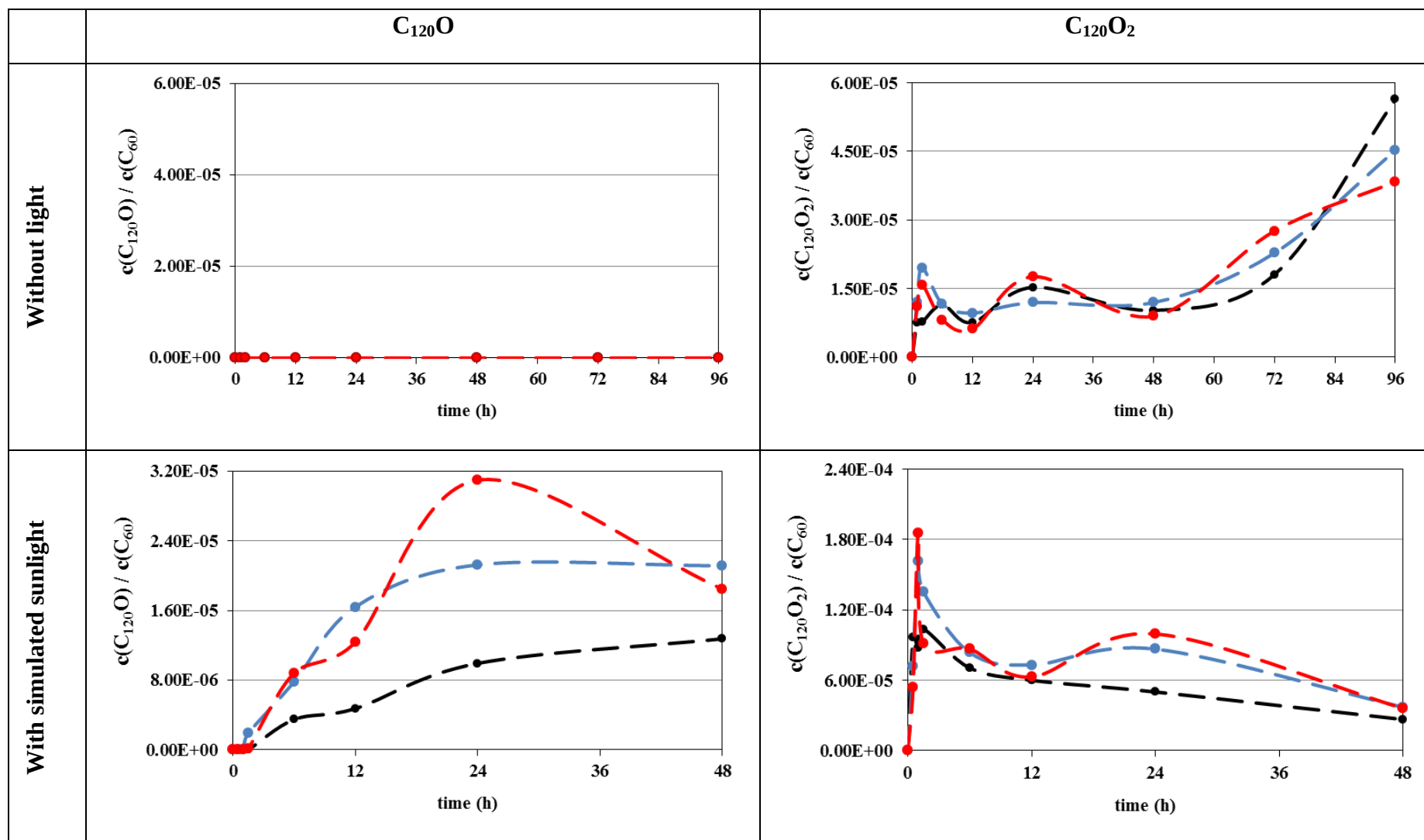
Figure S13 (cont). Impact of the humic acids content (●: [HA] = 0 \text{ mg l}^{-1} ; ●: [HA] = 2.25 \text{ mg l}^{-1} ; ●: [HA] = 0.30 \text{ mg l}^{-1} ) on the generation of selected C_{120}O_x .
