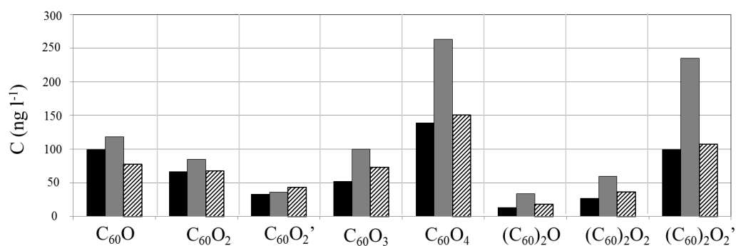
1 Figure 4. Occurrence of degradation products of C_{60} fullerene after 48 hours of simulated 2 sunlight irradiation in ultrapure water (black bars), in artificial freshwater (grey bars) and in 3 artificial seawater (dashed bars). The concentrations of degradation products were estimated 4 semi-quantitatively, because of the absence of commercially available analytical standards, 5 considering that they had the same response factor than C_{60} fullerene.
