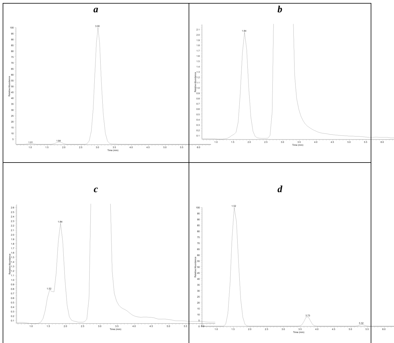
Figure S8. Signals of fullerenols observed in suspensions after sonication. Figure a shows a total ion chromatogram with three principal groups of signals: the peak of C 60 fullerene ( t_R=3.00 ), a peak of overlapped fullerenols at ( t_R=1.84 ) and unretained peaks near the dead volume ( t_R=1.01 ). The extracted ion chromatograms of [C 60 O] ·- , [C 60 O 2 H] ·- and [C 60 O 6 H 5 ] ·- are shown in Figure b , c and d .
