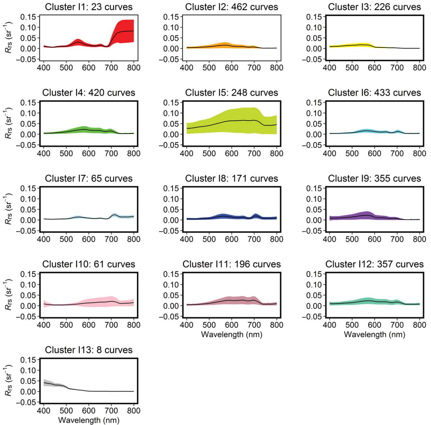
Fig. 6. Mean (solid black line) remote sensing reflectance ( R_{rs} ) and standard deviation (shaded area) obtained in inland waters as were identified by k -means algorithm. [Color figure can be viewed at wileyonlinelibrary.com ]
