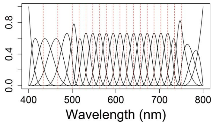
Fig. 3. Unequally spaced basis of B -spline functions (25) used in the study to fit the smooth curve. [Color figure can be viewed at wileyonlinelibrary.com]
