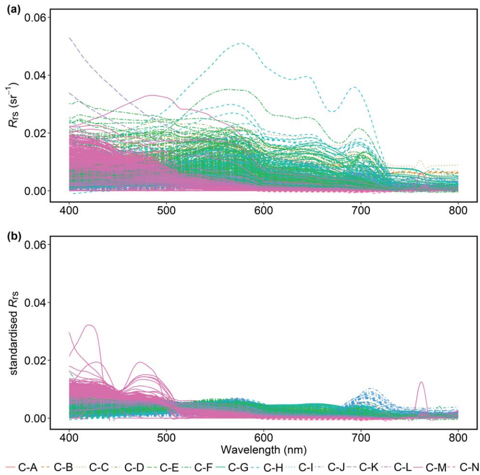
Fig. 2. In situ hyperspectral remote sensing reflectance spectra ( R_{rs} ) of datasets (Table 3) collected at coastal systems (a) on their original scale (b) standardized. [Color figure can be viewed at wileyonlinelibrary.com]
