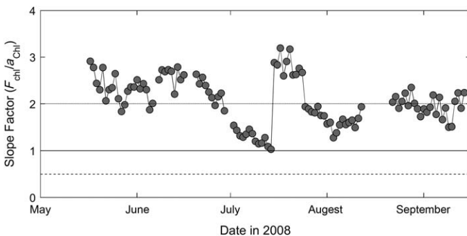
Fig. 6. Time series observations of the absorption-based slope factor derived from paired estimates of [Chl] from factory calibrated Chl fluorescence and a_{c9} absorption line height (Roesler and Barnard 2013) for 4 months in 2008. Data were collected from mooring D02 as part of the Gulf of Maine Ocean Observing System (GoMOOS) in Harpswell Sound, Casco Bay. Lines indicate slope factors of 0.5 (dash), 1 (solid), and 2 (dotted).
