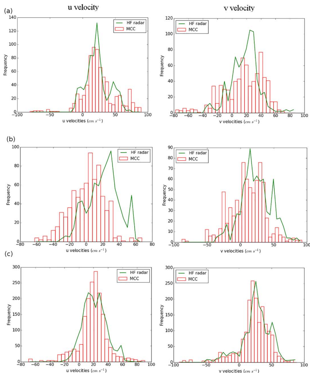
Figure 8. Distributions of MCC (red bars) and corresponding HF radar-derived (green line) current velocities in (left) u and (right) v directions. Data are for (a) nLw_412, (b) nLw_660, and (c) chlorophyll, all with time periods of 3, 4, 5, 6, and 7 h. All data are binned in 5\text{ cm s}^{-1} bins.
