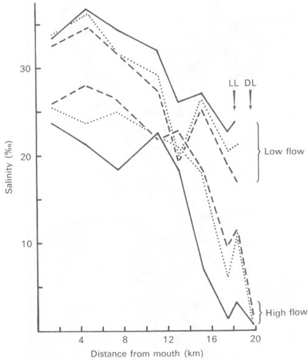
Fig. 2. Salinity of interstitial water in sediment. —, 0–5 cm depth; ···, 10–15 cm; ----, 15–20 cm. Upper lines are based on results from October 1969 when monthly mean river flow 3.56 m 3 /s following prolonged dry weather; lower lines on results from January 1970 when monthly mean river flow 63.6 m 3 /s. Arrows show upper limits of distribution of live Scrobicularia plana (LL) and of animals which appeared to have died in situ (DL).
