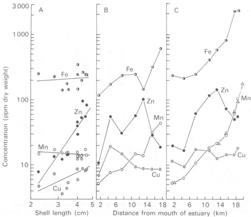
Fig. 8 (A) Effect of shell length on metal concentrations in scrubbed shells from 11 km station in October 1970. Slopes ( m ) for linear regression equation, \log_{10} concentration = m \log_{10} shell length + \log_{10} intercept, are: Zn, 3.425; Cu, 1.102; Mn, -0.115; Fe, 0.166; of which the first two are significantly different ( P < 0.05 ) from a slope of zero. Points are for single shells over 4 cm length, or, for smaller shells, pooled samples of 2-3. (B) Concentrations of metals in scrubbed shells from October 1970. Each point is a mean from five shells. (C) Concentrations of metals in washed shells collected at four seasons during 1969-70. Each point represents about 40 shells. \Delta , Manganese concentrations in buried shells of animals which appeared to have died in situ .
