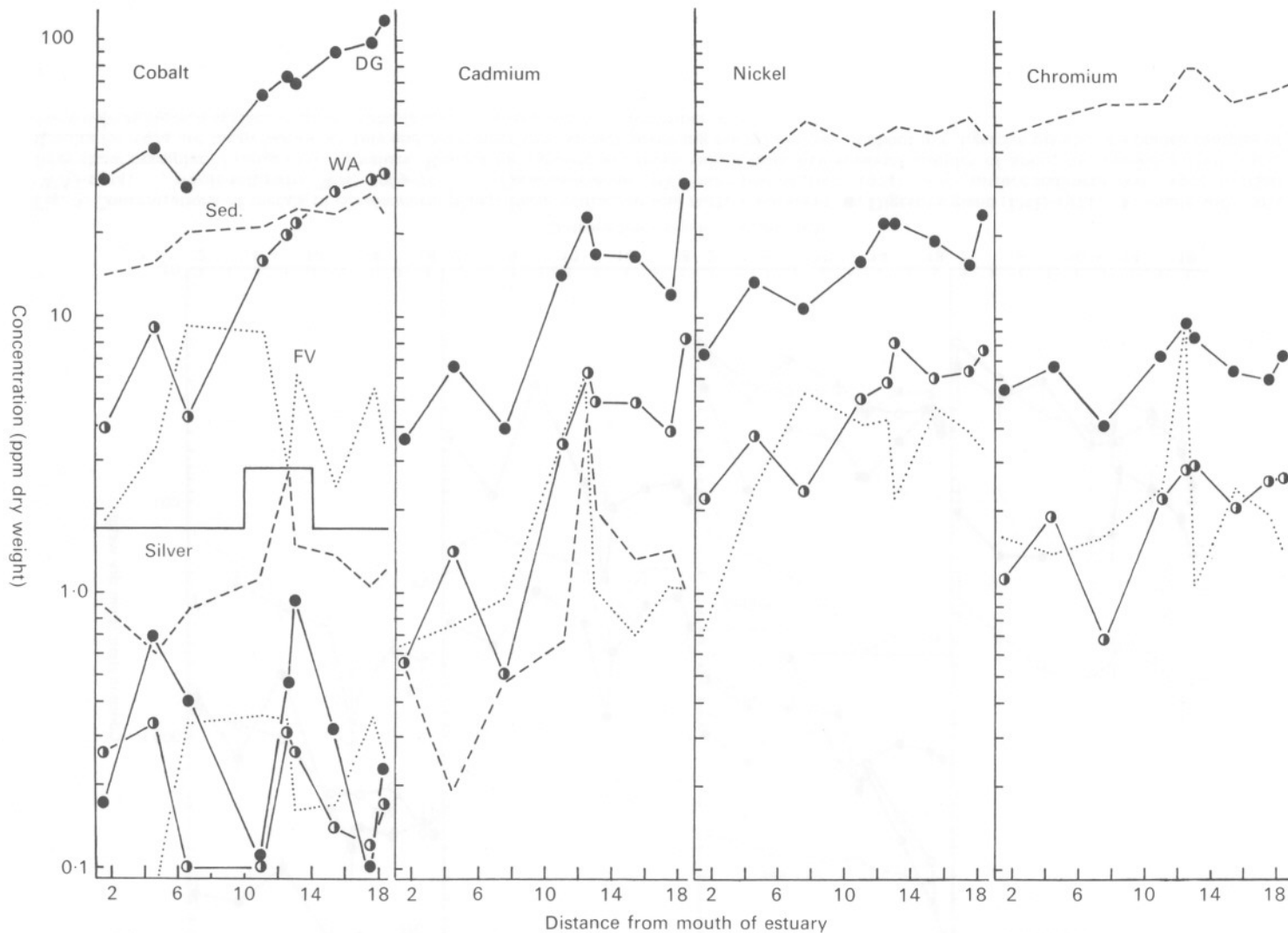
Fig. 4. Concentrations of metals in Scrobicularia plana , Fucus vesiculosus and surface sediment (cont.). For legend, see Fig. 3.
