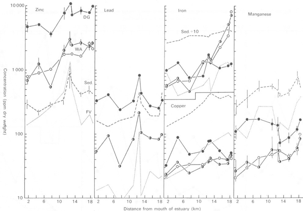
Fig. 3. Concentrations of metals in Scrobicularia plana , Fucus vesiculosus and surface sediment. ●, Digestive gland (DG)-1974; ○, whole soft parts (WA)-1974; ○, whole soft parts (WA)-1969-70; ···· Fucus vesiculosus (FV)-older thallus, Nov. 1974; ----, surface sediment (sed.)-1974. Vertical lines show examples of range of 1974 values. Results for 1969-70 are mean values from five seasonal samples of about five pooled animals each. Results for 1974 are mean values for July and November surveys each involving pooled samples of about five digestive glands, two pooled samples of five whole animals, a surface sediment sample and a seaweed sample (November only).
