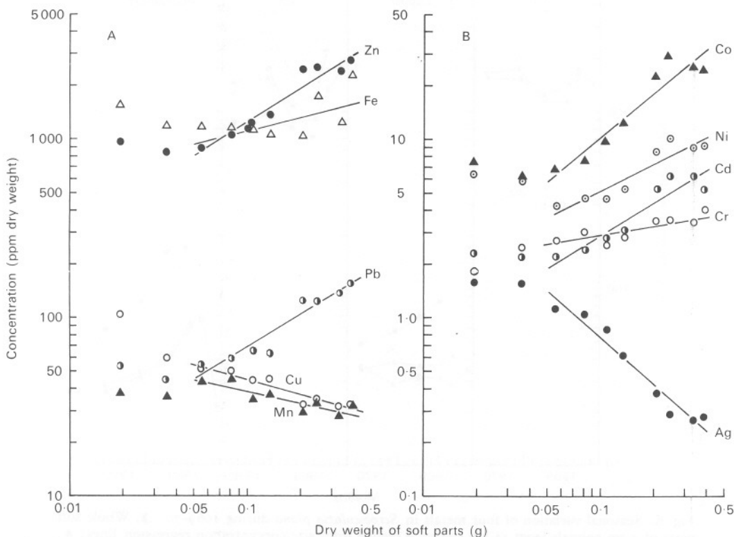
Fig. 5. (A & B). Relationships between concentrations of ten metals and the dry weight of the whole soft parts of Scrobicularia plana at 12.5 km station in Feb. 1975. For animals over 0.05 g dry weight, slopes ( m ) for the linear regression equation, \log_{10} \text{concentration} = m \log_{10} \text{weight} + \log_{10} \text{intercept} , are: Ag, -0.857 ; Cd, 0.606 ; Co, 0.817 ; Cr, 0.188 ; Cu, -0.280 ; Fe, 0.241 ; Mn, -0.215 ; Ni, 0.505 ; Pb, 0.603 ; Zn, 0.639 . Each point represents about five pooled animals.
