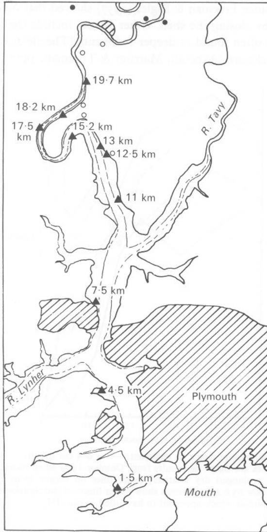
Fig. 1. Tamar estuary showing sampling stations (▲) with distance from mouth in km. Also shown are sites of some old lead mines (○) and copper mines (●). Based on the 1:25 000 Ordnance Survey Map with the sanction of the controller of H.M. Stationery Office, Crown copyright reserved.
