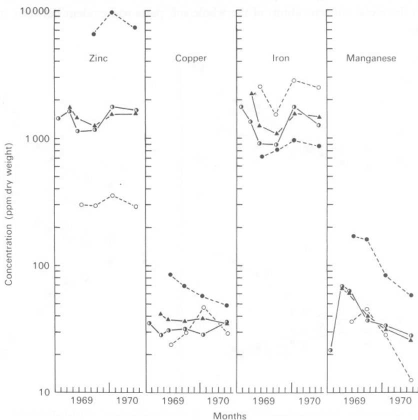
Fig. 6. Seasonal variation of four metals in Scrobicularia plana during 1969–70. ●, Whole soft parts of 4 cm animals from 11 km station – results from size/concentration regression lines; ▲, mean values for whole soft parts of animals from all 7 stations between 1.5 and 17.5 km; ●, digestive gland; ○, mantle/siphons from 11 km station – samples pooled from 10 animals.
