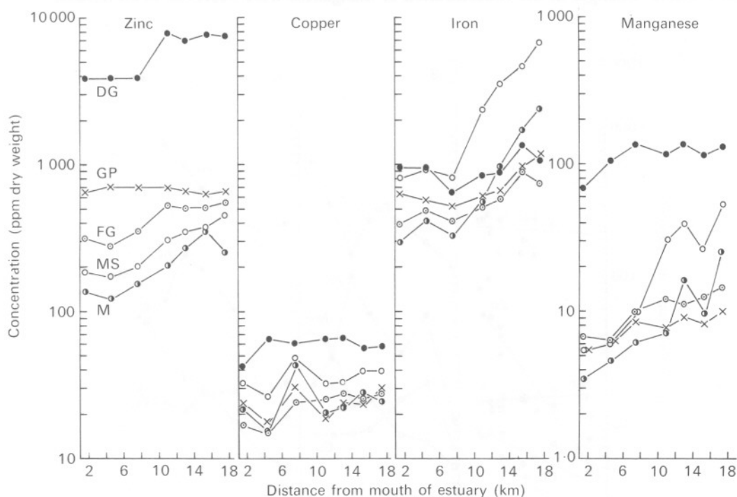
Fig. 7. Concentrations of four metals in tissues during 1969–70. Each point is a mean of four seasons and represents 40 animals. ●, Digestive gland; ×, gills and labial palps; ○, mantle and siphons; ○, foot and gonad; ●, adductor muscles. Contribution of tissues to dry weight of soft parts (including body fluid) was about 25% each for digestive gland, mantle/siphons and foot/gonad, about 7% for adductor muscles and 6% for gills/labial palps.
