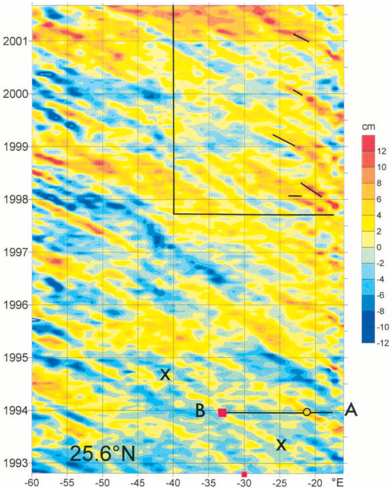
Figure 10. Hovmöller or travel contours for swesty -like anomalies along a path from 18° W to 60° W at 25.6° N after removing a mean annual signal to reveal more clearly the B -like anomalies (Figure 7). East of 18° W, the path followed is south from 27.5° N to 26.0° N along 17° W (see Figure 9). Swesty was followed continuously from ~25° W to ~41° W (marked by 'x') by Argos buoys. The line 'A' to 'B' shows the track of RRS 'Charles Darwin' along ~26° N to the eddy survey region (red square). Open circle at ~21° W marks the sea level anomaly about 12° to the east of swesty . Surface chlorophyll- a along A–B is shown in Figure 11. The red cross near 30° W indicates the October survey position of an open tracer release experiment. The window (top right) shows the overlap of altimeter and SeaWiFS data used in this study (see Figure 12).
