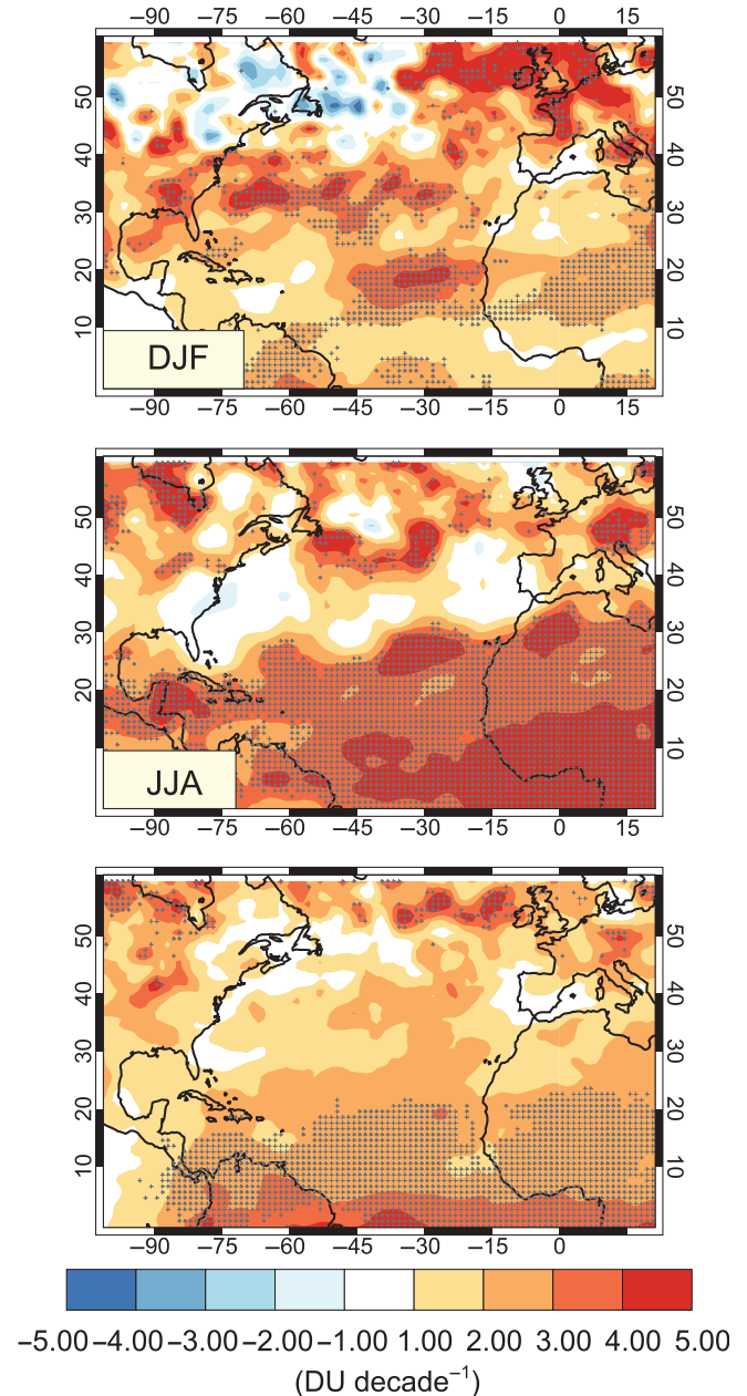
FIGURE 7 Decadal linear trends (ca. 2006–2016) calculated using seasonal (DJF [top] and JJA [middle]) and annual-mean (bottom) ozone tropospheric column. Trends are calculated over the period 12/2005–2/2016. The stippling indicates where trends are significant to the 95% confidence level, based on the standard error of the residuals (Wigley et al. , 2006). Methane trends show little variation spatially and seasonally (not shown) [Colour figure can be viewed at wileyonlinelibrary.com ]
