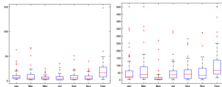
Fig. 3. Box plot for the time to discover a leak when the time series in the leak cell (left) and adjacent cell North of the leak (right) is used. The box represent first and third quartile, top and bottom are the 25th and 75th percentile of the samples, respectively. The median time to detection is shown by the red line inside the box. The whiskers extends to 1.5 the interquartile distance, measurements outside of the whiskers represent outliers and are shown as red crosses.
