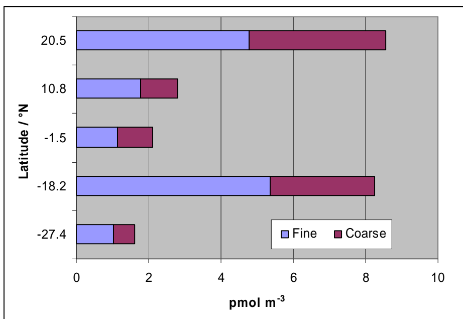
Figure 10. Preliminary data showing iodide concentrations in the fine ( <1\mu\text{m} ) and coarse ( >1\mu\text{m} ) particles of 5 aerosol samples collected during AMT13.
